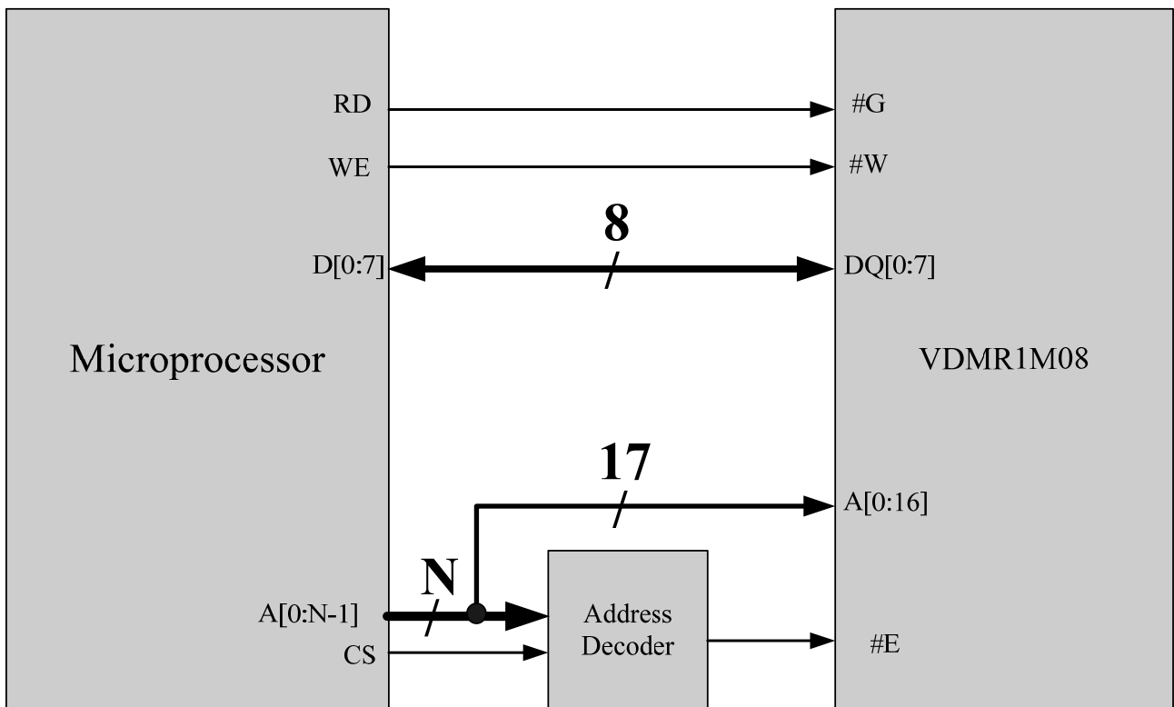
Figure 3 Typical application
