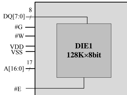
Figure 1 Block diagram
