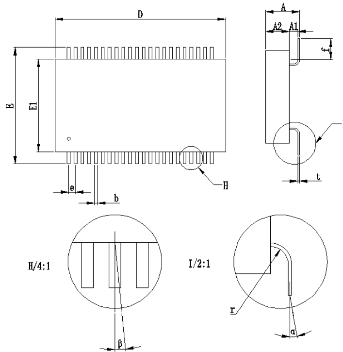
Figure 4 Package dimensions
